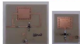
12 GHz SIW oscillators
