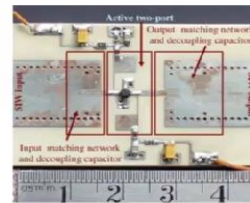
X-Band SIW amplifier
